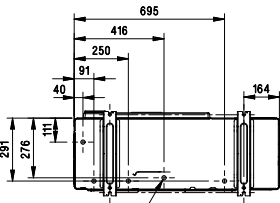
5-L.D. 20 holes for drain connection
